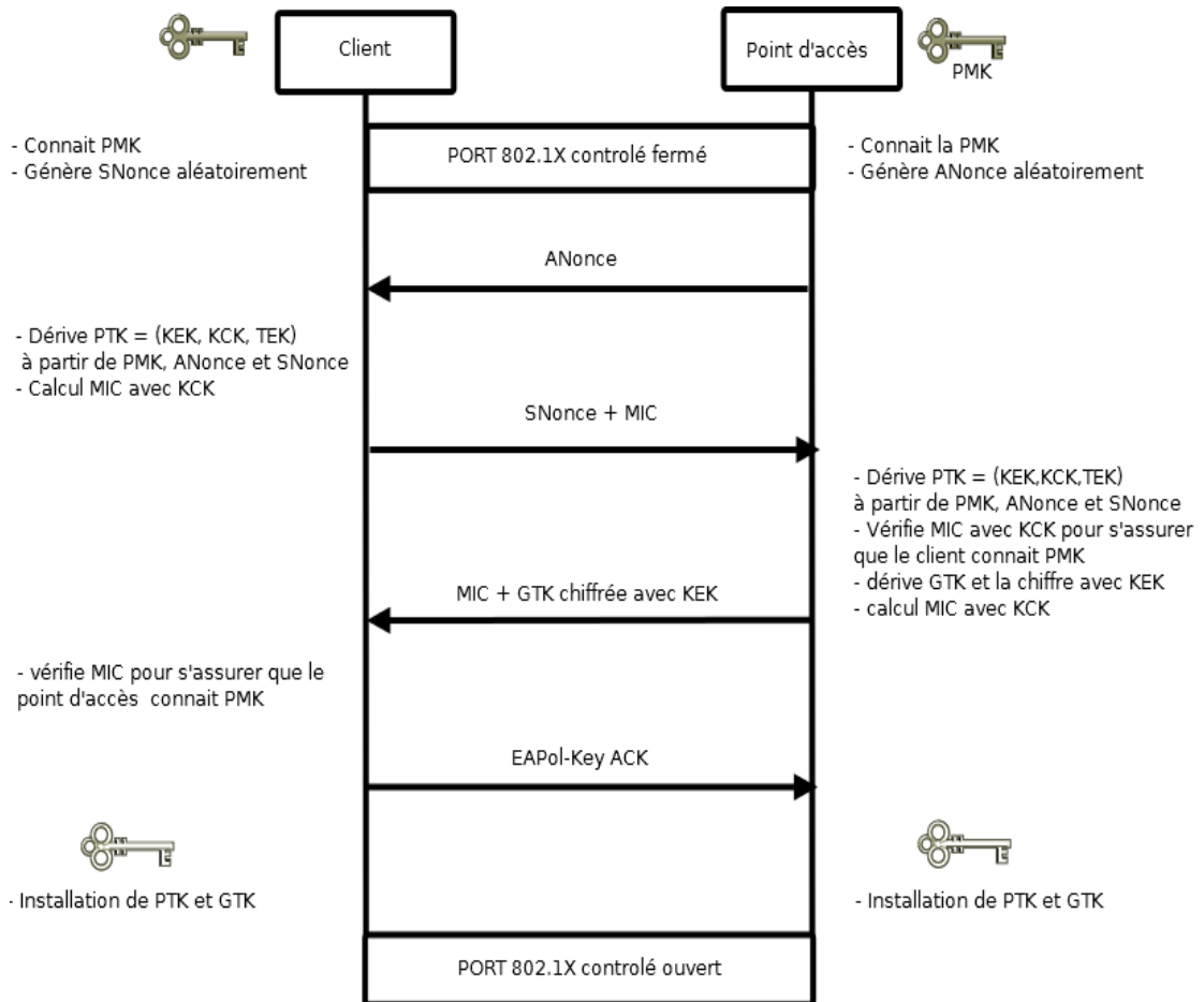
Figure 6 : 4 way handshake
